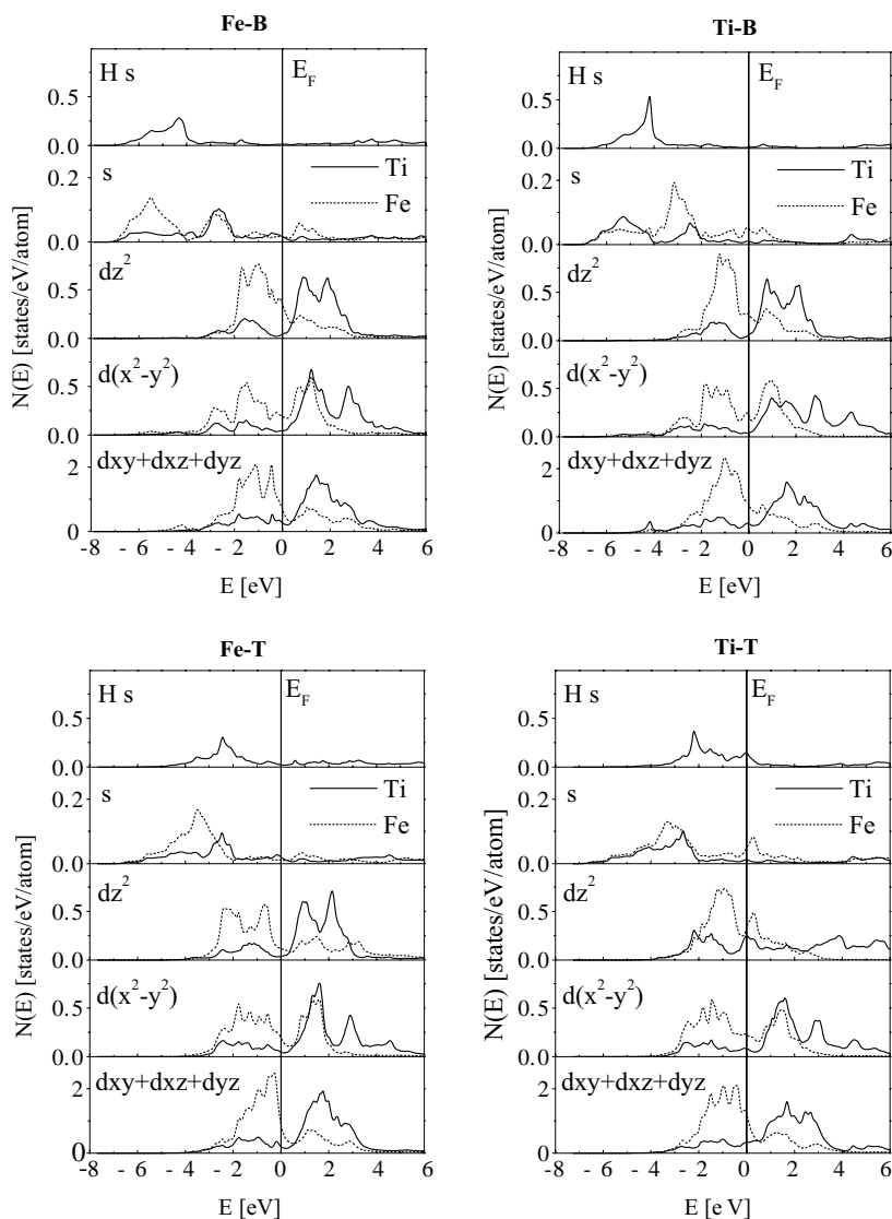
Fig. 8. Partial DOS in the surface layer of substrate in TiFe (110) films with H in Ti-B, Fe-B, Ti-T, Fe-T position, respectively.
