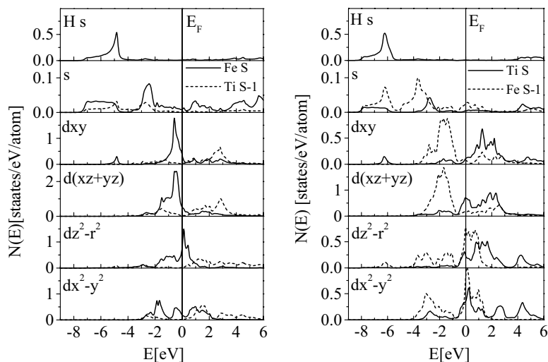
Fig. 5. Partial DOS in the surface (solid lines) and subsurface (dashed lines) layers of the substrate and on the adsorbate H site for H/TiFe (001) with H atom in the “hollow” position.
