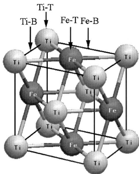
Fig. 6. The calculated H adsorption sites on the TiFe (110) surface. Ti-T and Fe-T denote H adsorbed on-top of Ti or of Fe atoms and Ti-B and Fe-B mark H adsorbed on a bridged site between Ti or Fe atoms.
